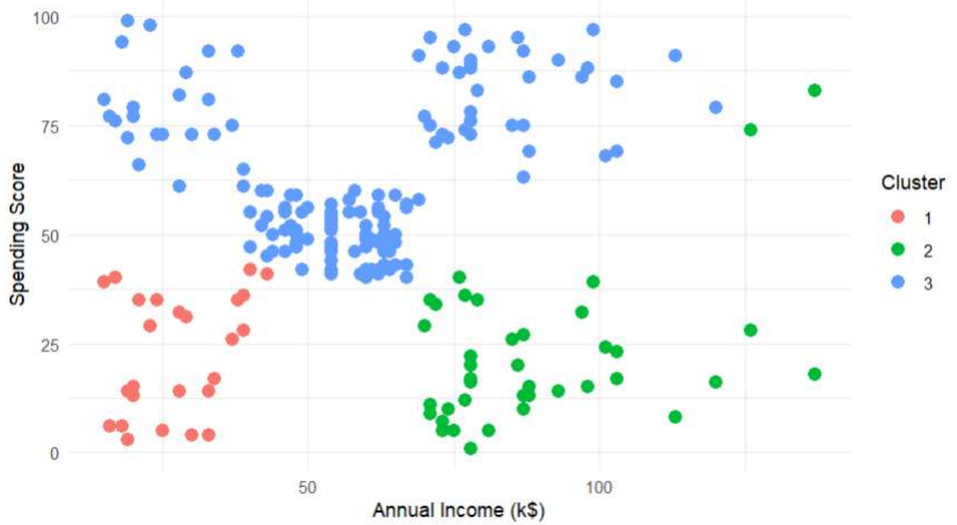
Customer Segmentation using K-Means Clustering
